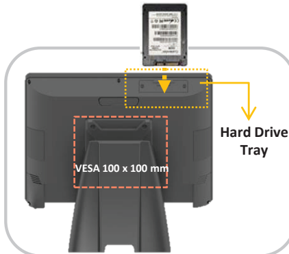
Easy access hard drive tray Support VESA mounting
